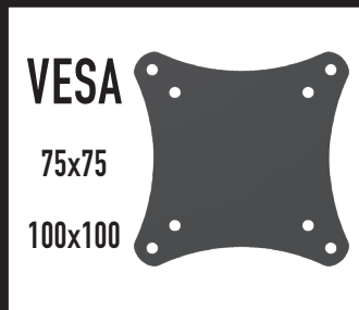
VESA Hole Pattern
